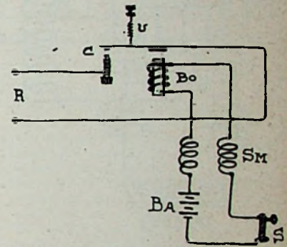
Fig. 2. Relay.
